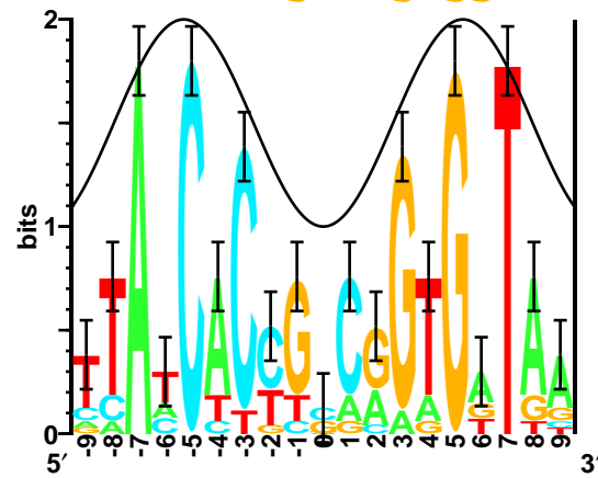
12 Lambda cI and cro binding sites
