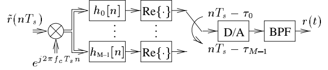
(a) Modulation using periodically nonuniform reconstruction
