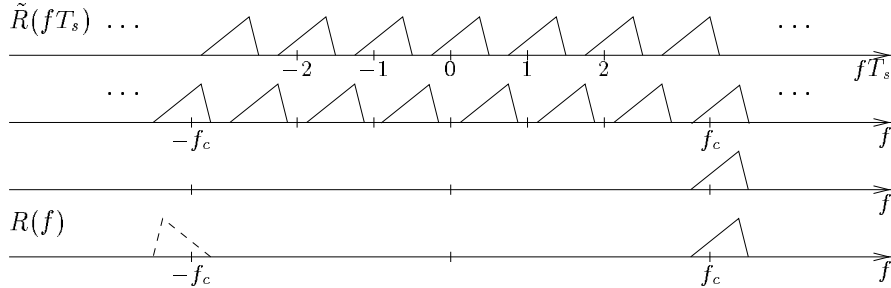
(b) Example signal spectra for the modulator of Fig. 4(b).
