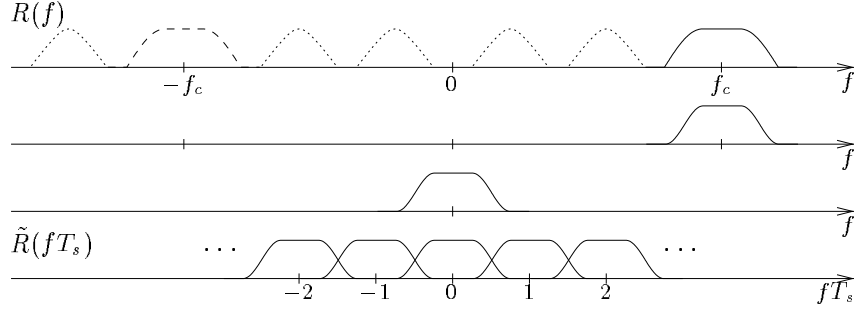
(a) Example spectra for the demodulator of Fig. 1(b) operating on a communication waveform, including spectral shaping and symbol-rate sampling.
